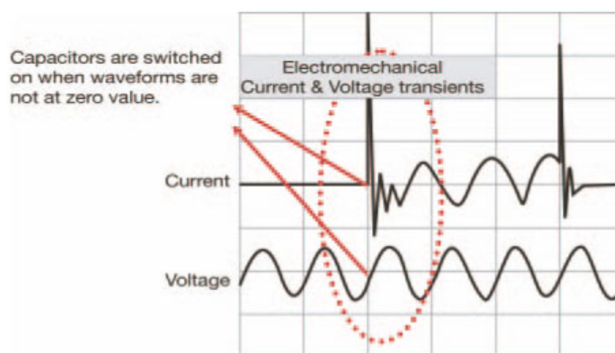
Electromechanical vs. Transient - free switching.
